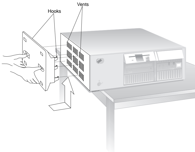
Figure 1-83. Floor Stand
