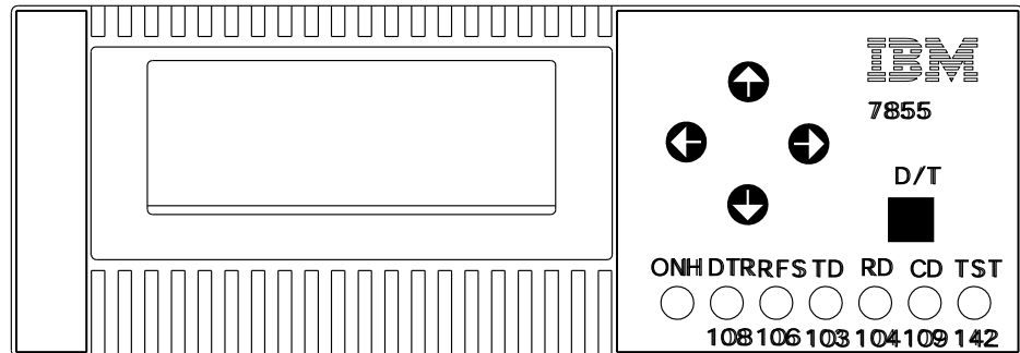
Figure C-1. 7855 Front Panel
