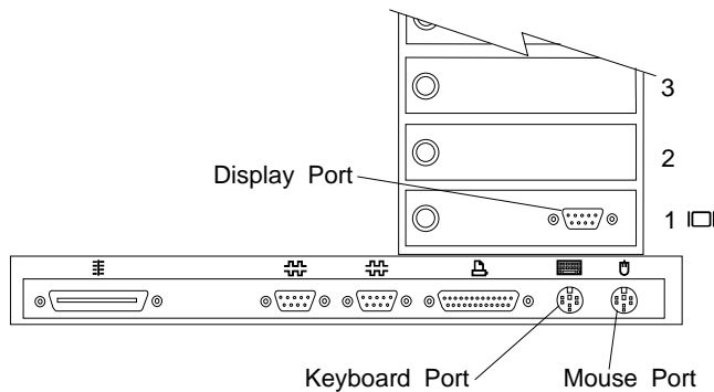
Figure 1-81. Cable Locations
