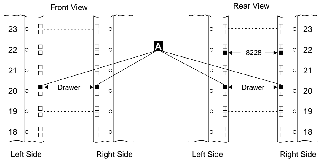
Figure 1-9. Installing Captive Nuts for the Service Drawer
