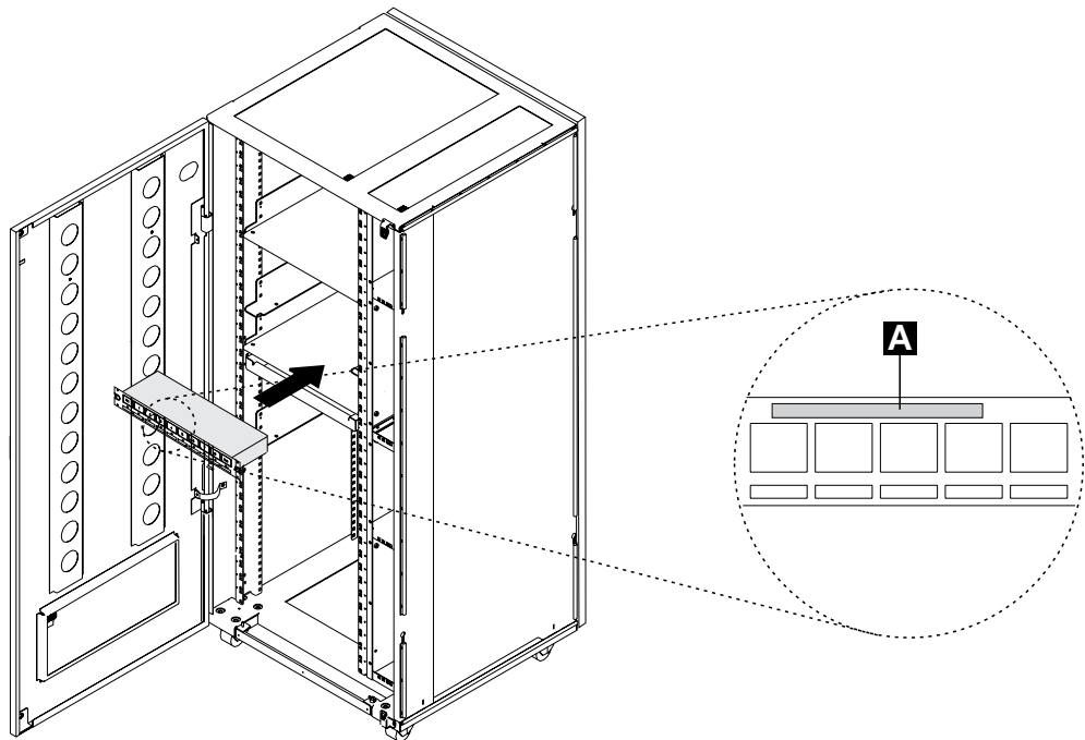
Figure 1-45. Installing the 8228 (Controller Expansion Rear side)
