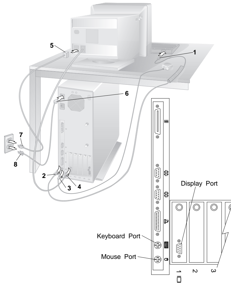
Figure 1-85. Cable Connections
